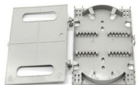
Model: FZ-YH09-24 Size:172*88*10.7
