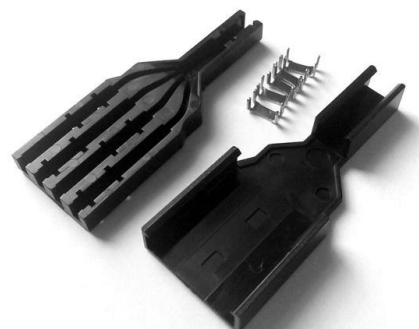
FTTH 4C fanout kit
